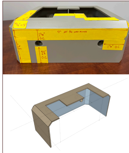
Patio part drawing converted into CAD drawing with SketchUp software.
